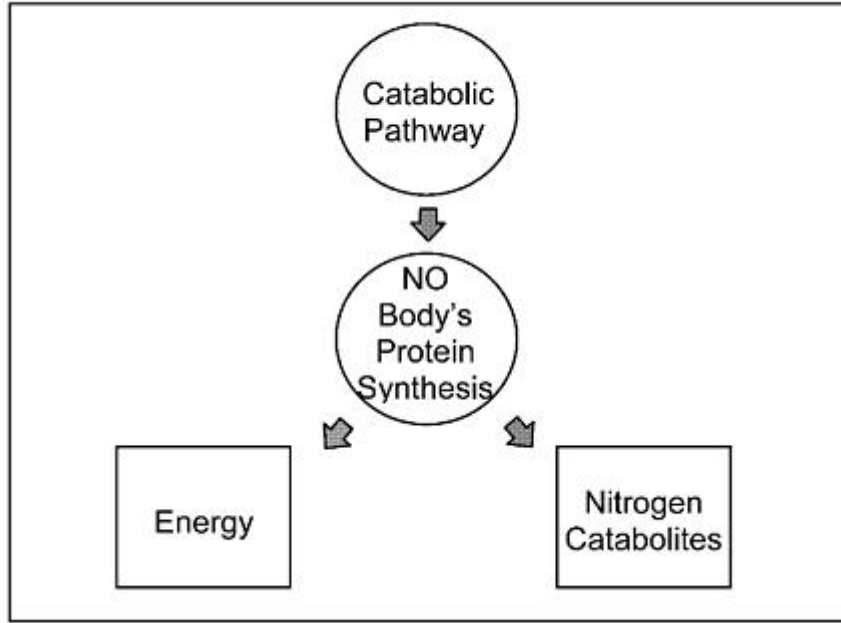
Figure III. The Protein Metabolism Catabolic Pathway
